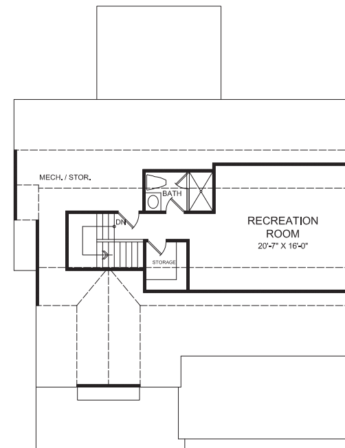
THIRD FLOOR
